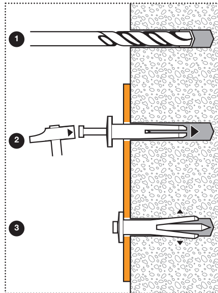
Fast all metal hammer fixing
